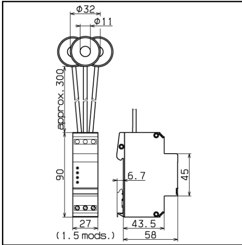
Dimension drawing DISO 3
